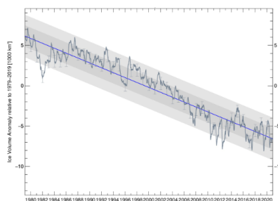
Polar Ice Loss Tripled in Last Decade
