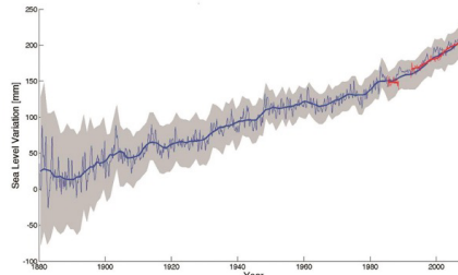
Sea Levels Risen by 20cm in Past Century
