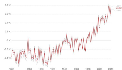
Global Temperatures 1.1°C Warmer Than Pre-Industrial Levels
